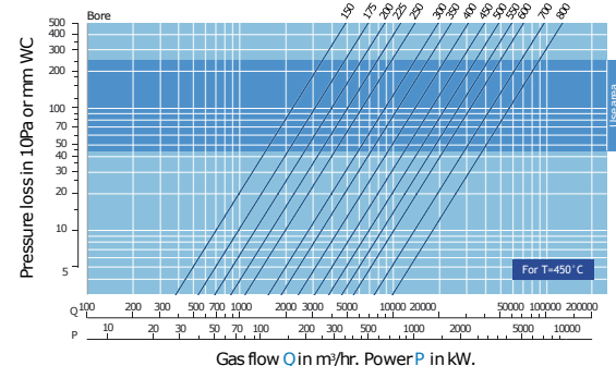
Silencer nominal diameter choice
