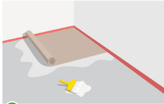
2 Underlay application (glued)
